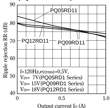
Fig.20 Ripple Rejection vs. Output Current (PQ05RD11 Series)
