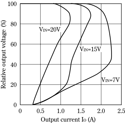
Fig. 4 Overcurrent Protection Characteristics (Typical Value)(PQ05RD11)
